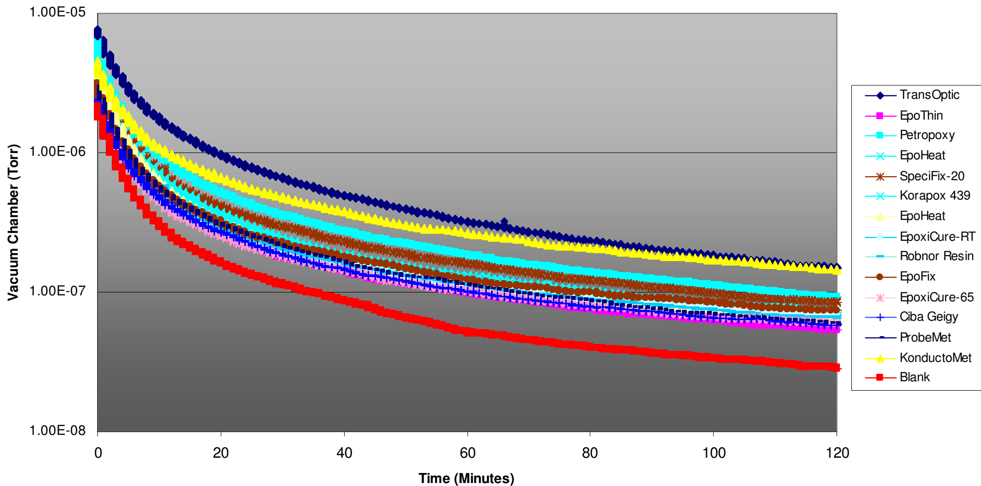
Total Pressure Pump Down - After 3 months Cure
